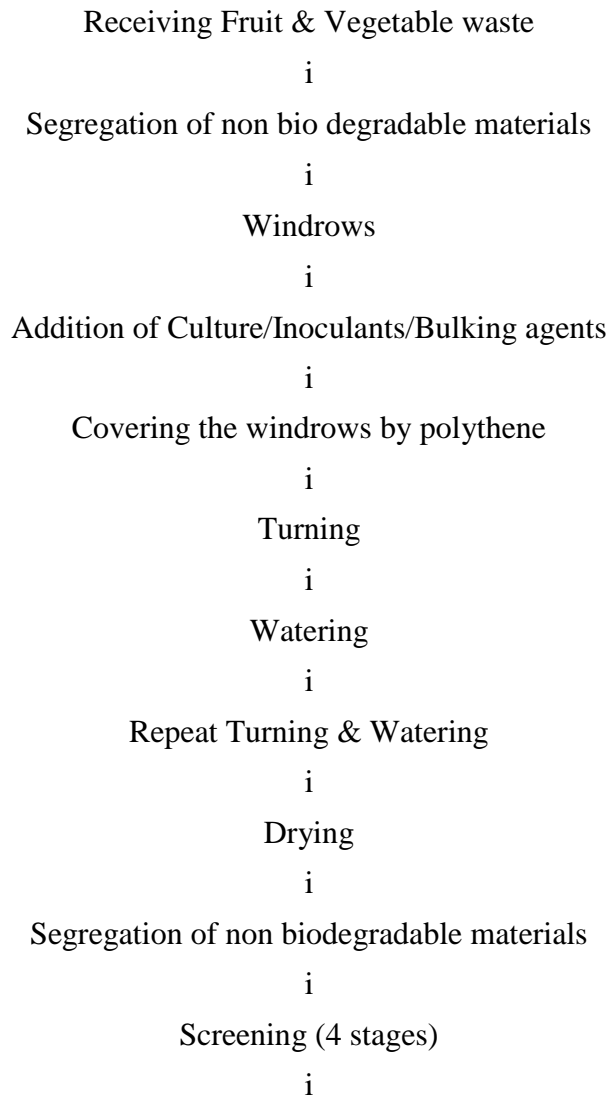
Fig. 1. Flow Diagram Showing Various Steps in Compost Production
